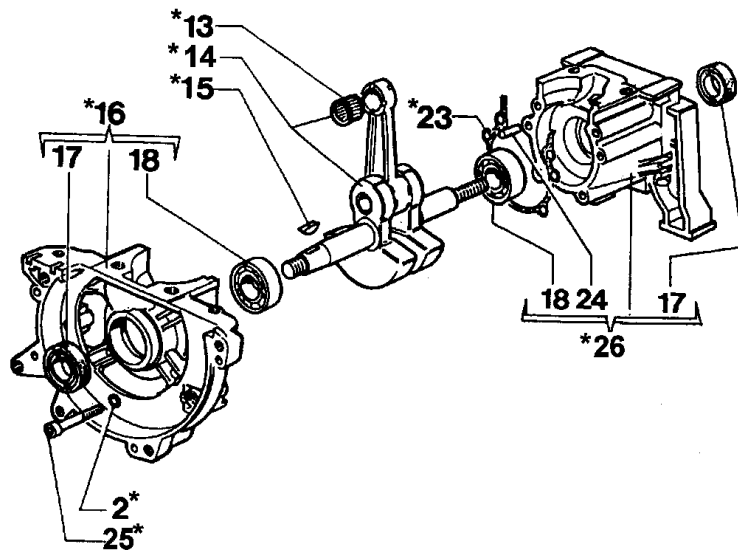
*27 Short Block
