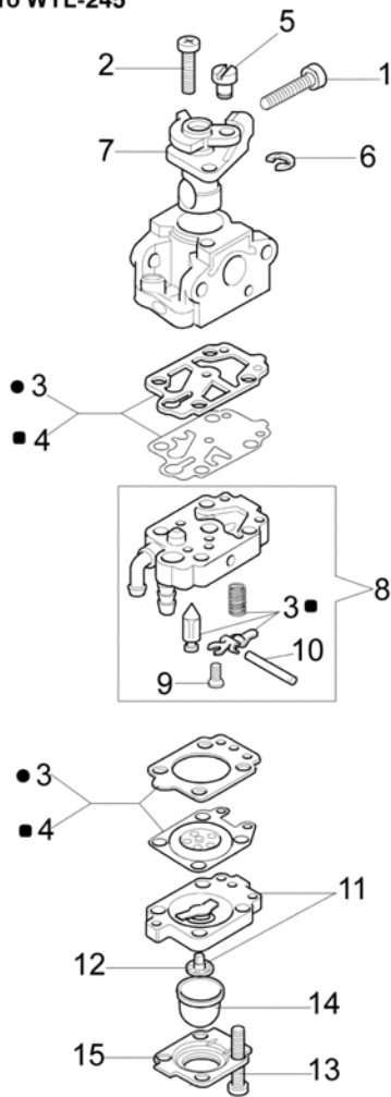
Walbro WYL-245
